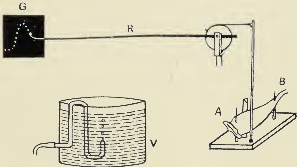
FIG. 176. The Peristaltograph.
